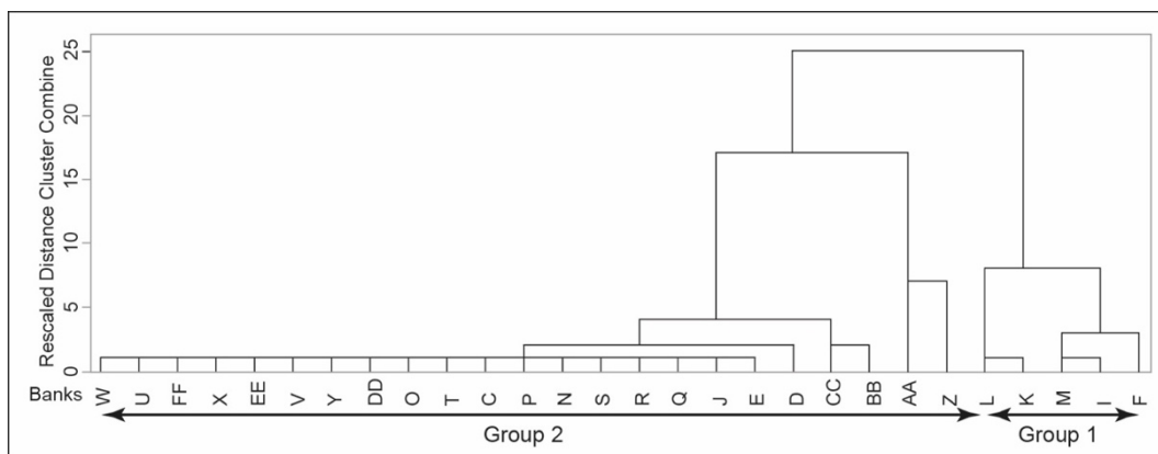
Figure 5: Dendrogram
