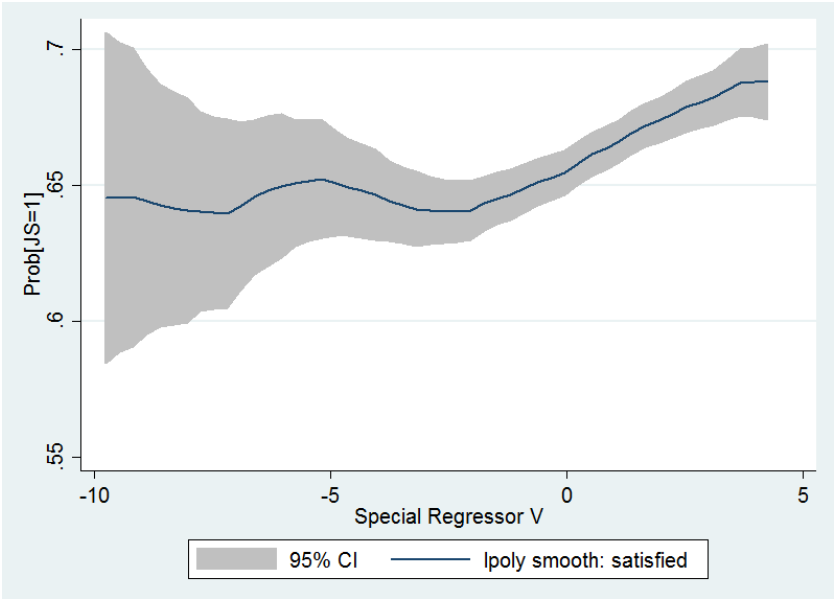
Figure 2.2: Kernel Weighted Local Polynomial Regression of JS on V
