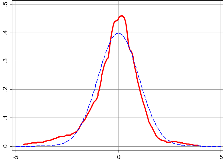
Figure 1. Underlying distribution.
