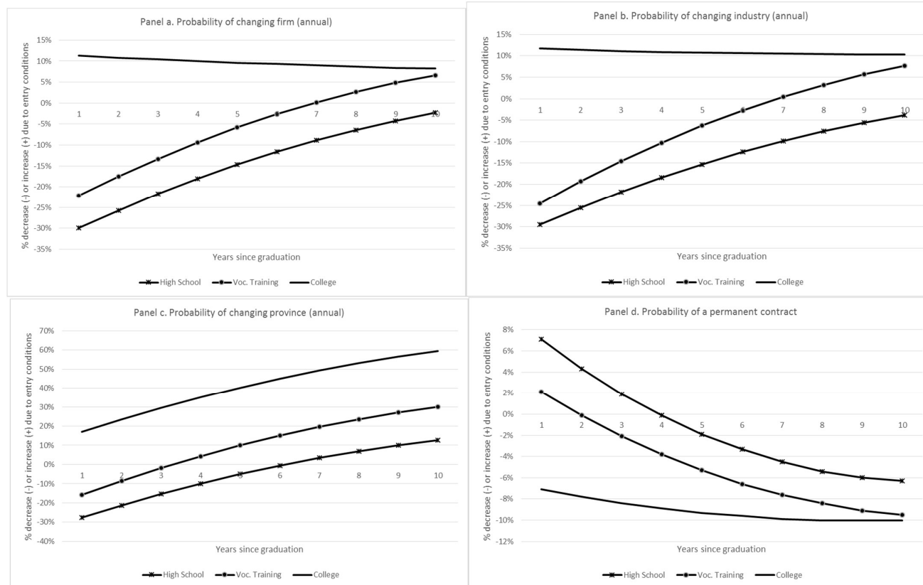
Figure 4: Persistent Effects of the Province Unemployment Rates the Year of Labor Market Entry on the: (1) Probability of Changing Firms (annual change); (2) Probability of Changing Industry (annual change), (3) Probability of Changing Province (annual change); and (4) Fraction with Permanent Contract
