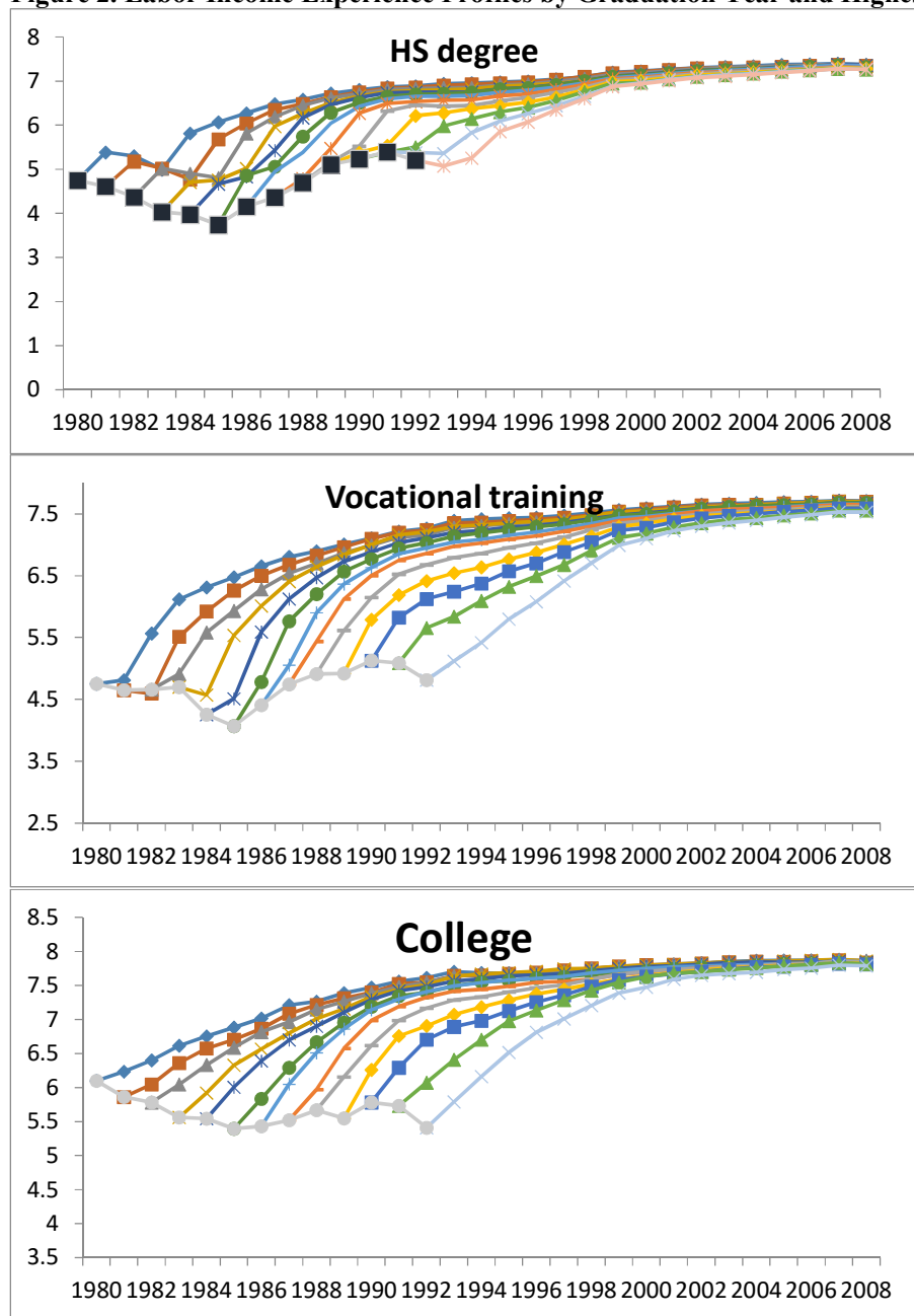
Figure 2. Labor Income Experience Profiles by Graduation Year and Highest Education Level
