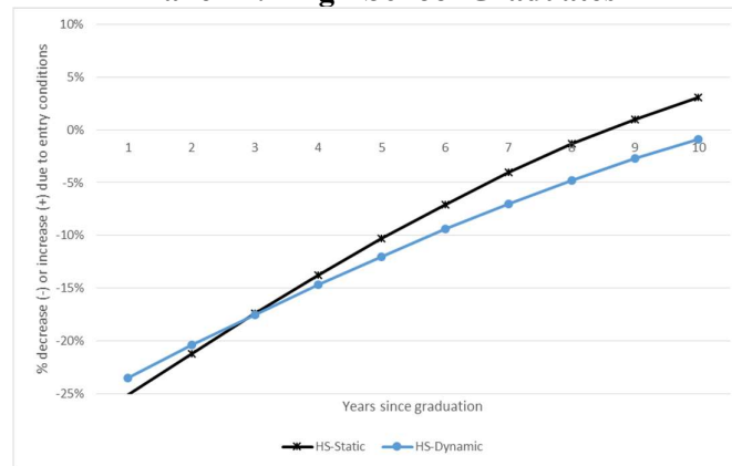
Figure 3. Persistent Effects of the Province Unemployment Rates the Year of Labor Market Entry on Annual Earnings Effect of a 8-ppt Rise in Unemployment Rate at Labor Market Entry Cohorts Graduating Between 1980 and 1992
