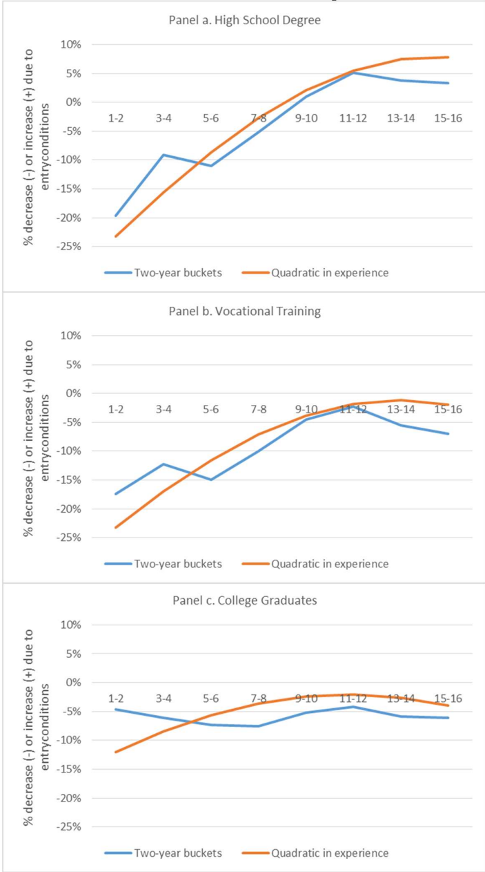
Figure A.1. Annual Earnings as a Function of Initial Conditions Second-Order Polynomial versus Two-Year buckets Experience (Full-Effects Specification) Effect of a 8-ppt Rise in Unemployment Rate at Labor Market Entry Cohorts Graduating Between 1980 and 1992
