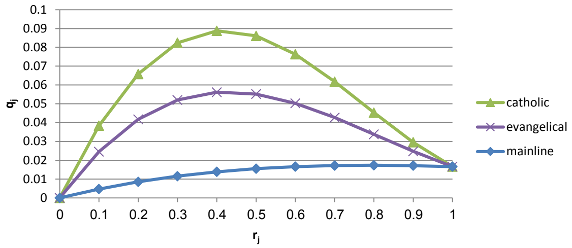
Figure A1: The relationship between q_j and r_j
