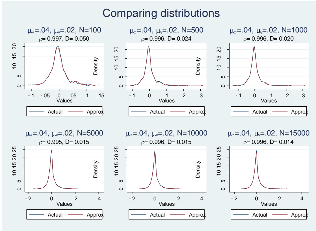
Figure 1d: Comparing the actual and the Taylor's series approximation of the error (Eq 11 vs. Eq 12)
