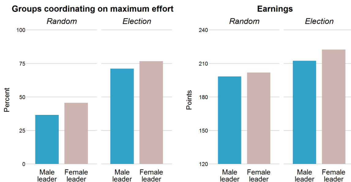
Figure 2. Fraction of teams that coordinate on the highest effort (left) and mean earnings per period (right) in periods 12 to 26 depending on the treatment and the gender of the leader.
