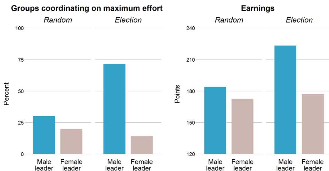
Figure 1. Fraction of teams that coordinate on the highest effort (left) and mean earnings per period (right) in periods 9 to 11 depending on the treatment and the gender of the leader.
