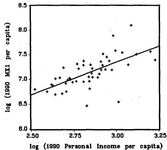
Figure 4d: MX1 and Personal Income, 1990 Cross-Section
