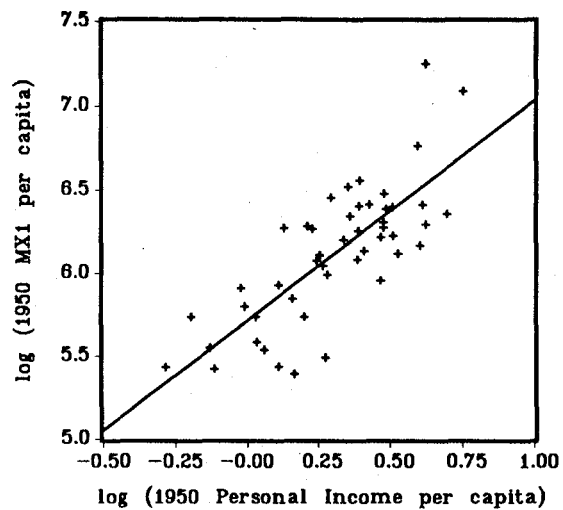
Figure 4b: MX1 and Personal Income, 1950 Cross-Section
