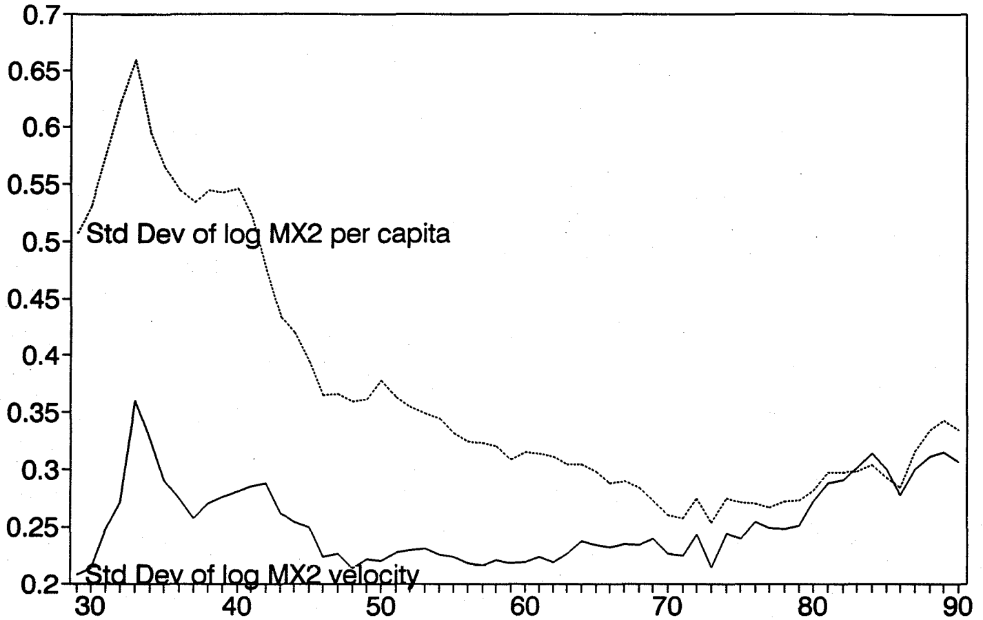
Figure 2: MX2 dispersion Cross-sectional Std Dev, 1929-90
