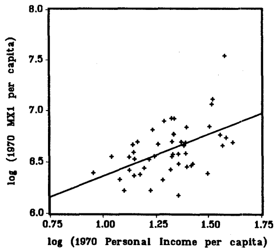
Figure 4c: MX1 and Personal Income, 1970 Cross-Section
