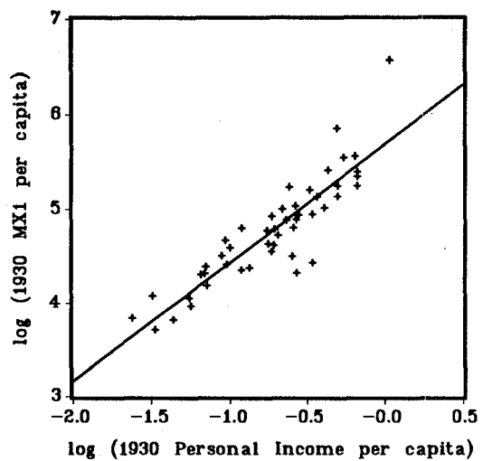
Figure 4a: MX1 and Personal Income, 1930 Cross-Section
