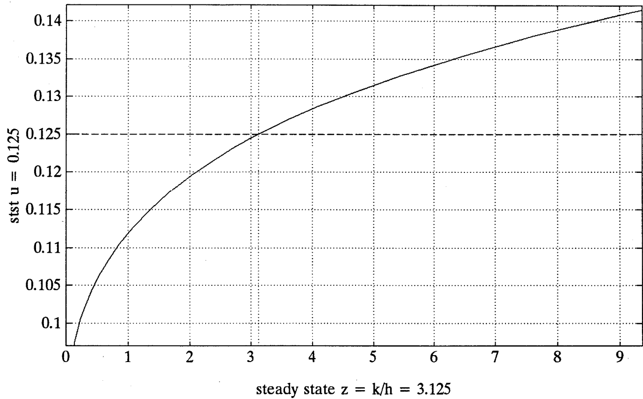
Fig 5(b). u(z) in the Lucas model. \theta < \alpha .
