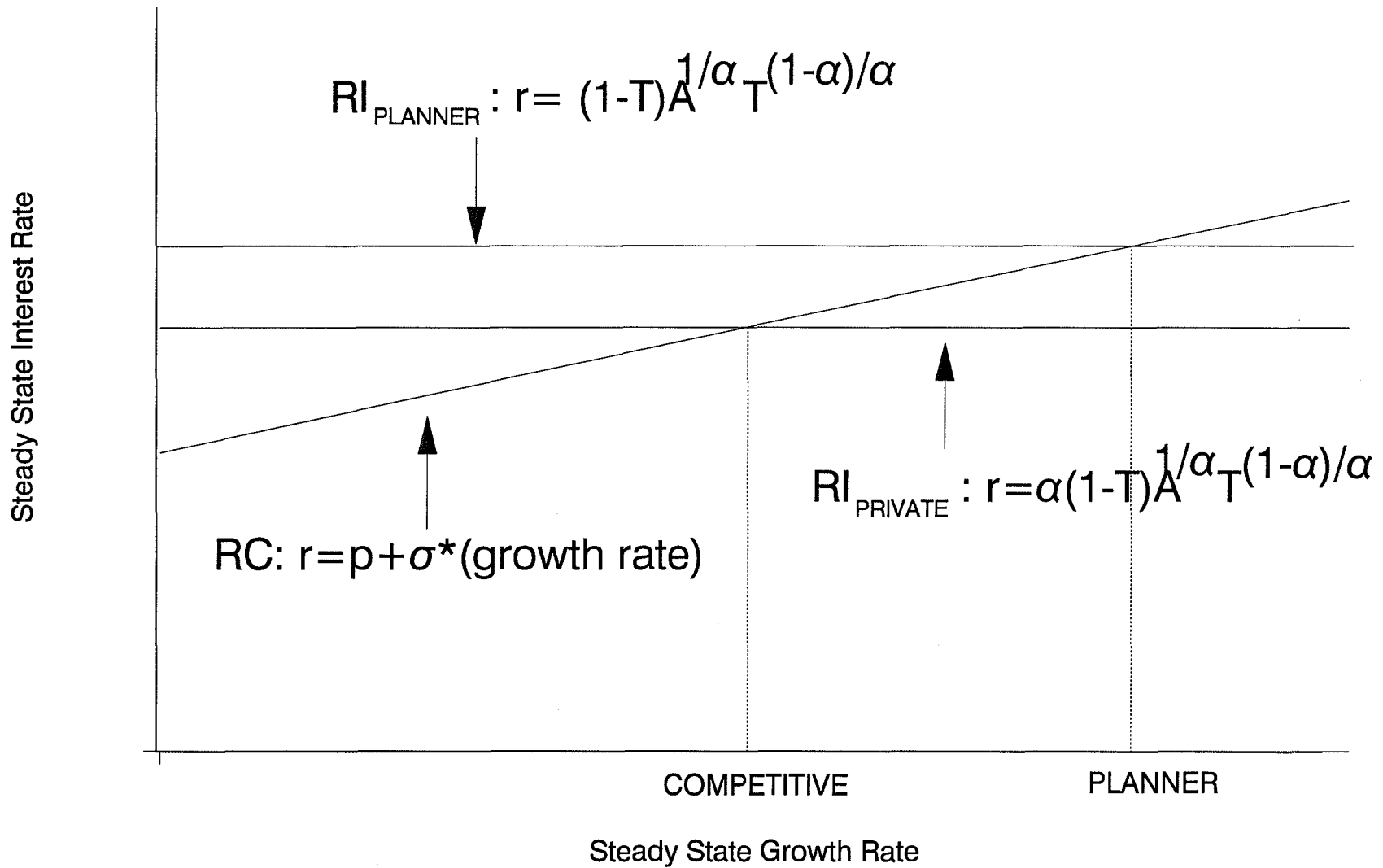
FIGURE 3: BARRO MODEL
