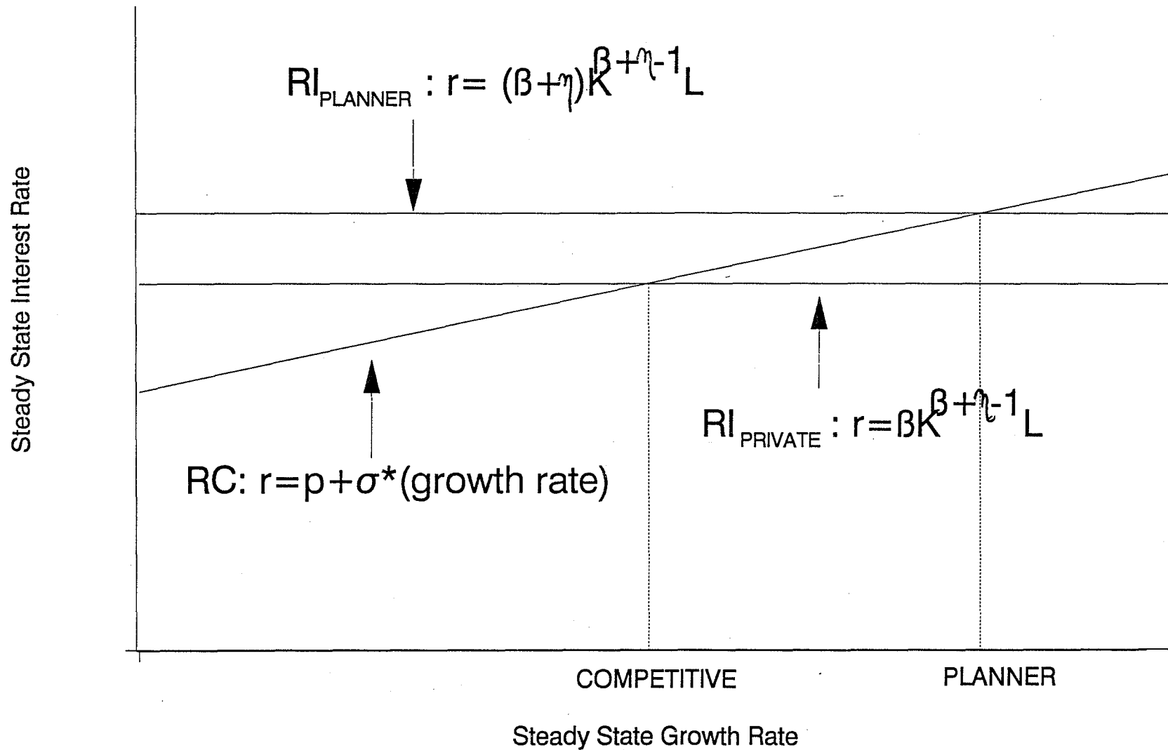
FIGURE 4: ARROW-SHESHINSKI-ROMER MODEL
