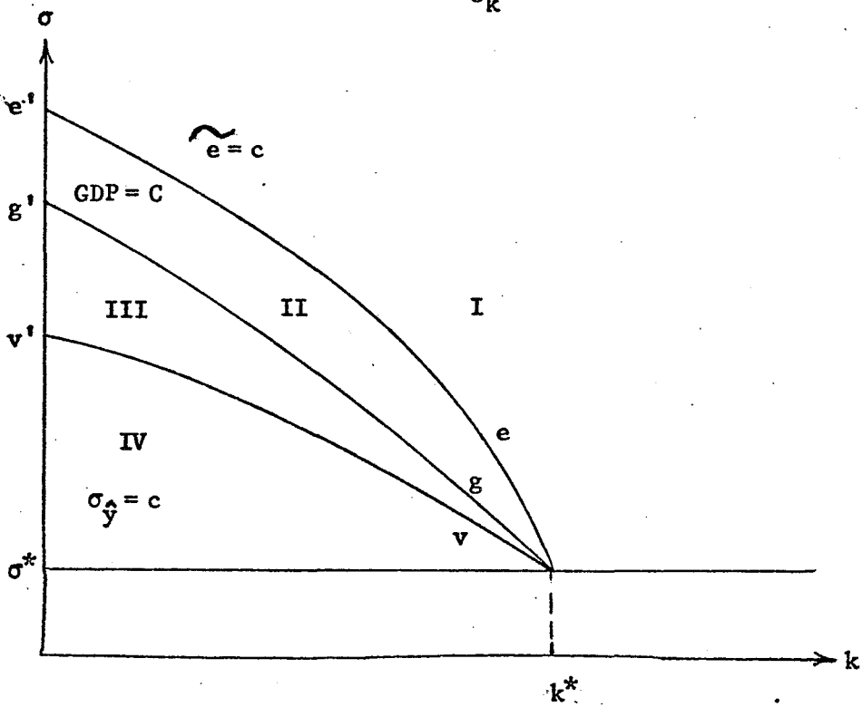
FIGURE 4. g_k < 0
