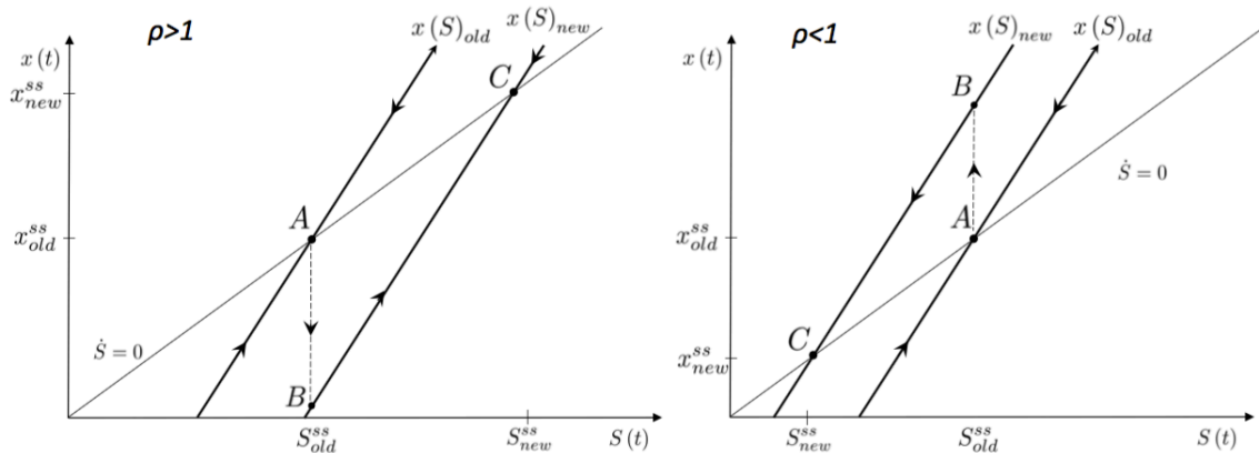
Figure 1: Short and long-run price effects. A permanent price increase makes the policy function x(S) shift downward for an impatient consumer ( \rho > 1 , left panel), and upward for a patient consumer ( \rho < 1 , right panel). Consumption of x on impact jumps from A to B , then it follows the new policy function x(S)_{new} until the new steady state C is reached.
