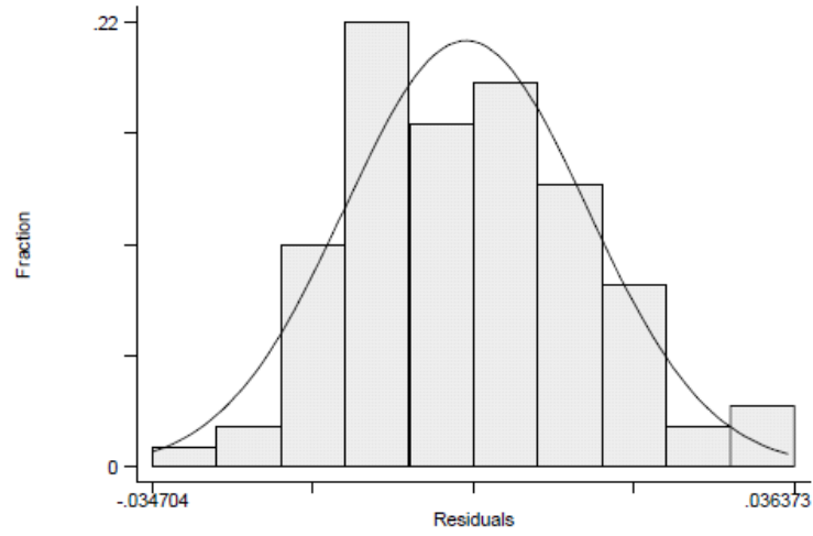
Figure 5: Residuals are independently and identically distributed as a normal N \sim (0, \sigma^2) in the case of the single popular externality effect
