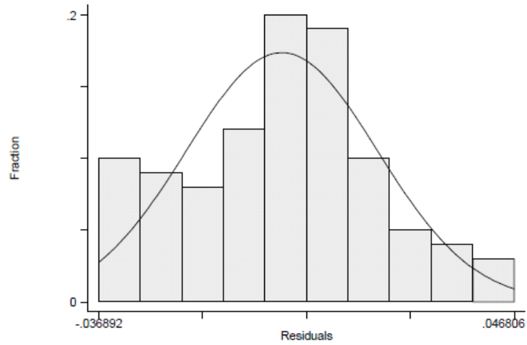
Figure 1: Residuals are independently and identically distributed as a normal N \sim (0, \sigma^2)
