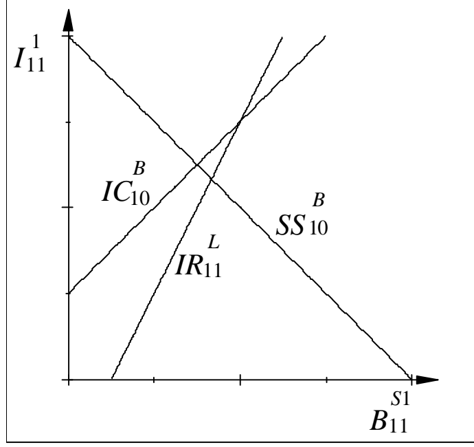
Figure 3: The three constraints in the third-best program The point where (IR_{11}^L) crosses (SS_{10}^B) is characterized by the system
