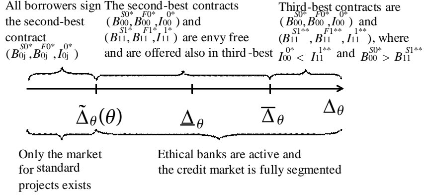
Figure 2. Moral hazard and screening (third-best): given the relative expected returns of standard and ethical projects, third-best contracts depend on the magnitude of the premium for successful interaction as illustrated in Proposition 2
