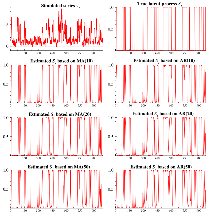
Figure 6: Simulation Study: True vs. estimated posterior probability Pr(S_t = 1 | \mathbf{Y}) . On the two upper panels the simulated time series y_t and the true (simulated) latent process. On the lower panels the estimates of Pr(S_t = 1 | \mathbf{Y}) based respectively on the MA(10) , MA(20) and MA(50) approximation.
