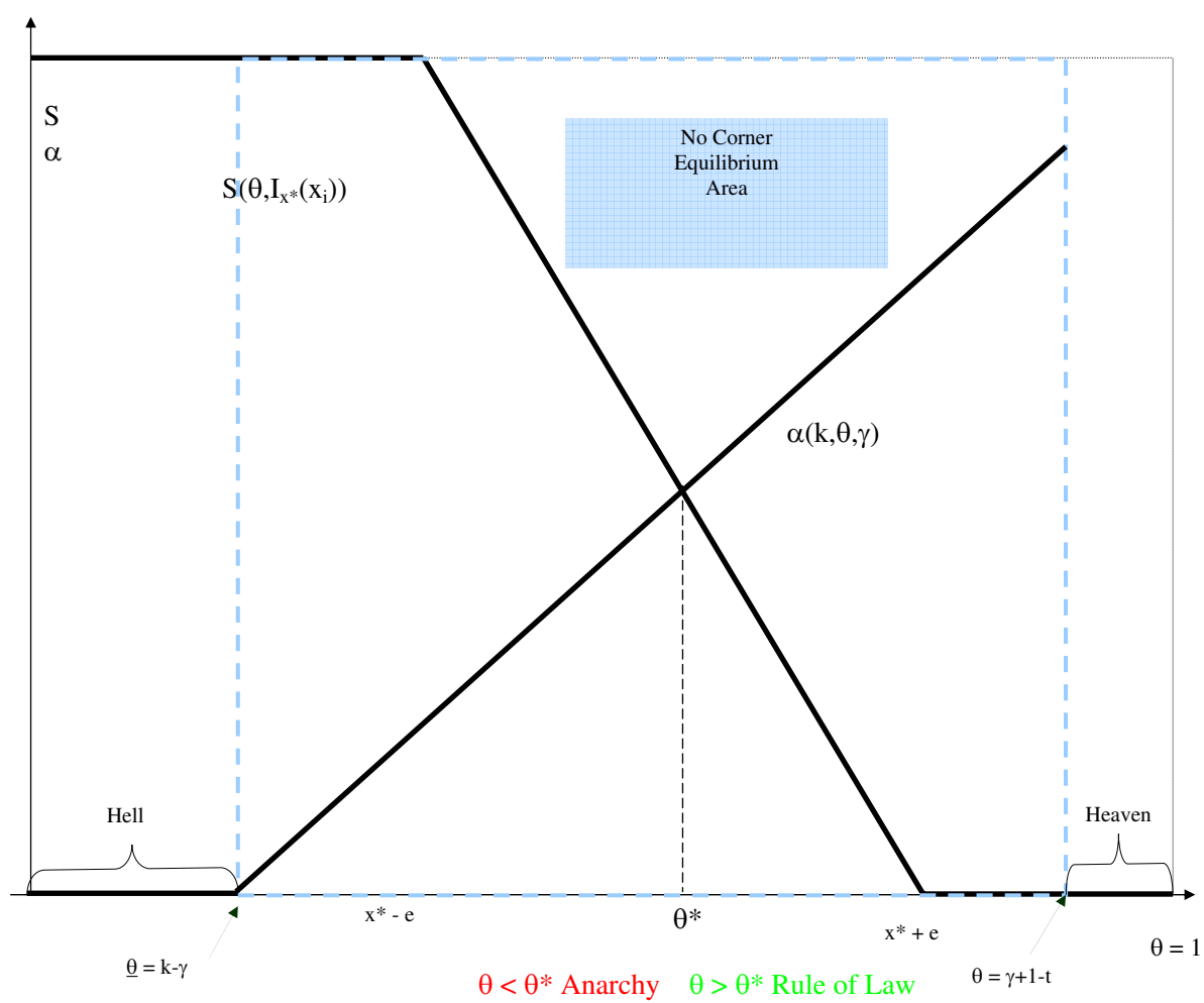
Figure 7: Equilibrium: \theta^*
