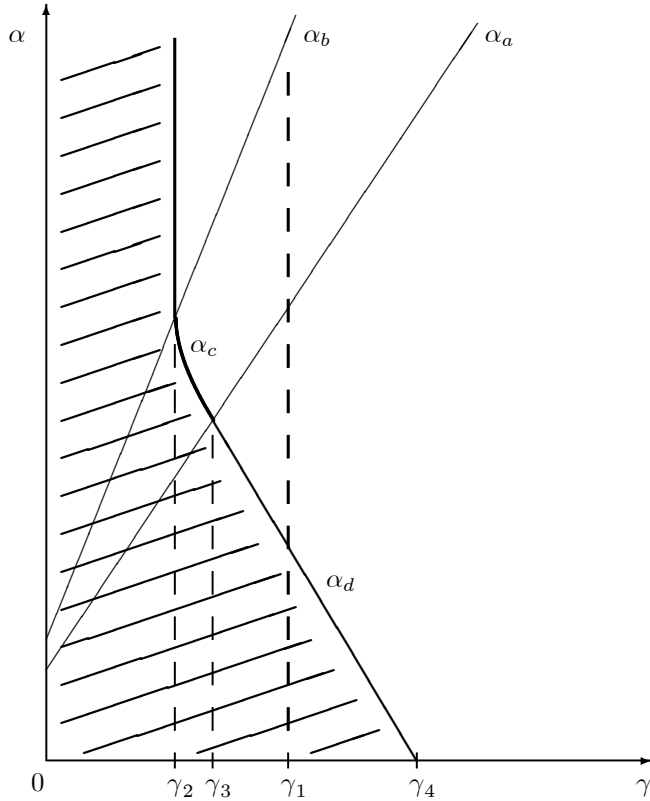
Figure 4 : The equilibrium (0,0)
