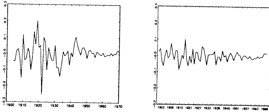
Fig. 18. Residuals obtained from a DS model with p=2 (left), and a ST model with m=12 local time trends (right), plotted in the same scale.
