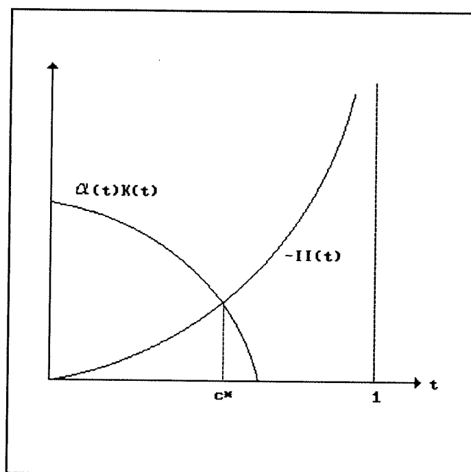
Figure 1: Proposition 1
