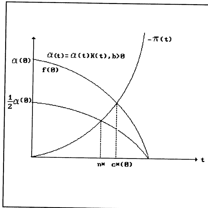
Figure 3.2: Proposition 5(ii)
