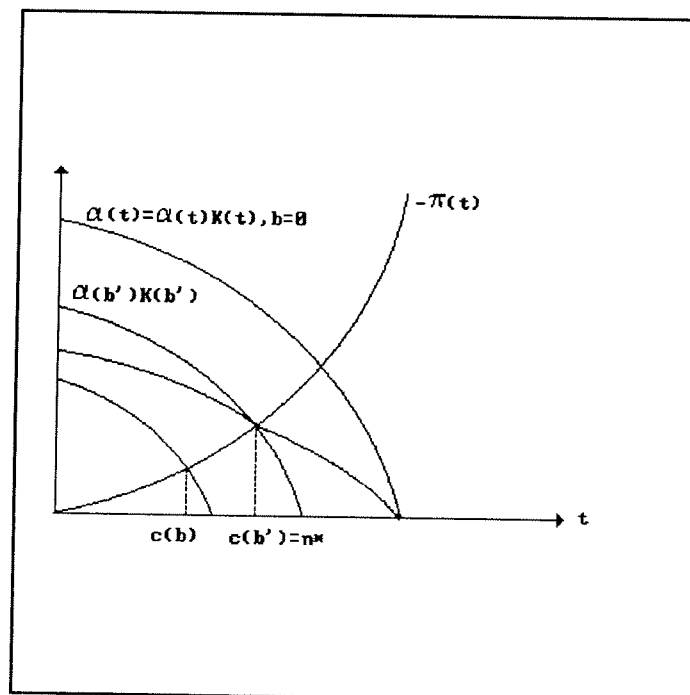
Figure 3.2: Proposition 5(ii)
