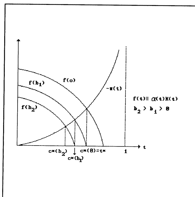
Figure 2.1: Proposition 2(i)
