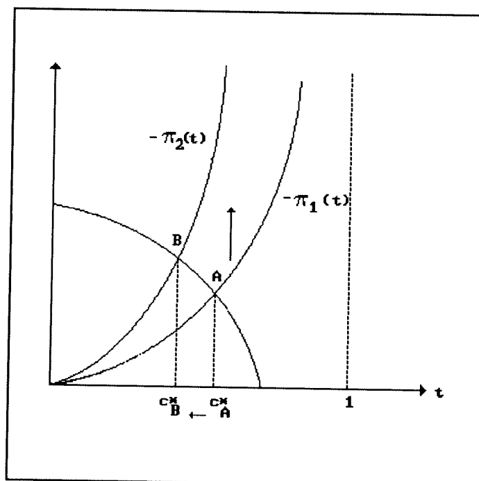
Figure 2.3: Proposition 2(iii)
