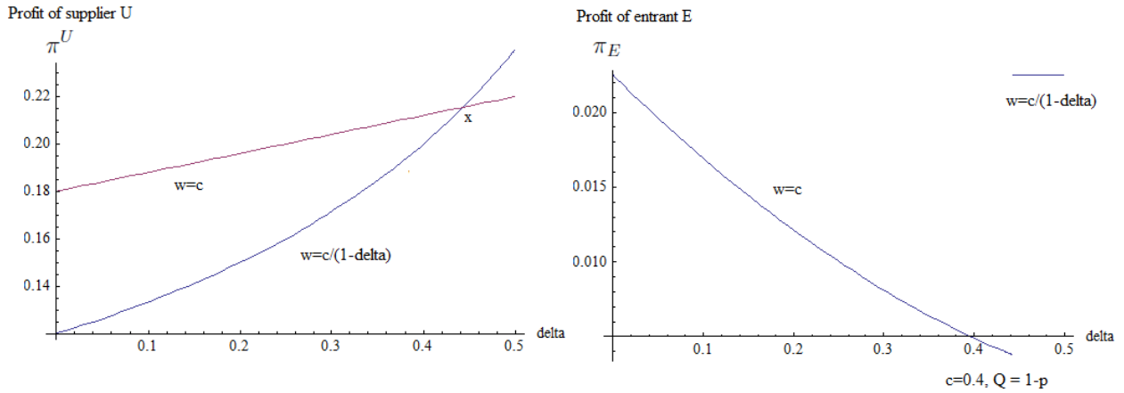
Figure 1: Profits as a function of the incumbents' non-controlling backward ownership
