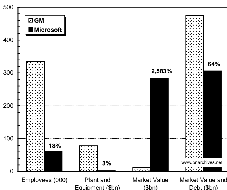
Figure 3: General Motors versus Microsoft, 2005
