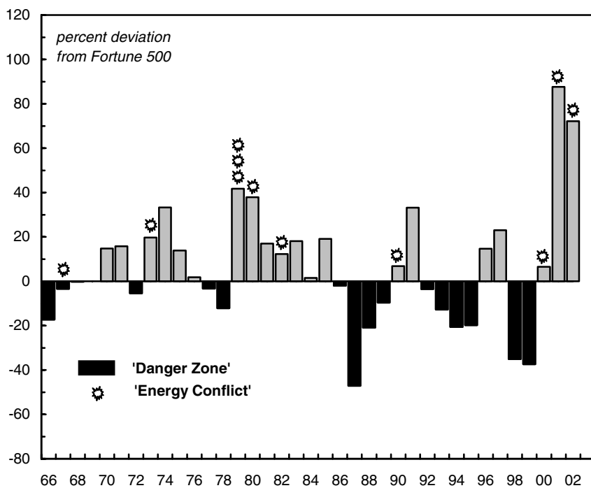
Figure 14 – The Petro-Core’s Differential Accumulation* and Middle East ‘Energy Conflicts’**
