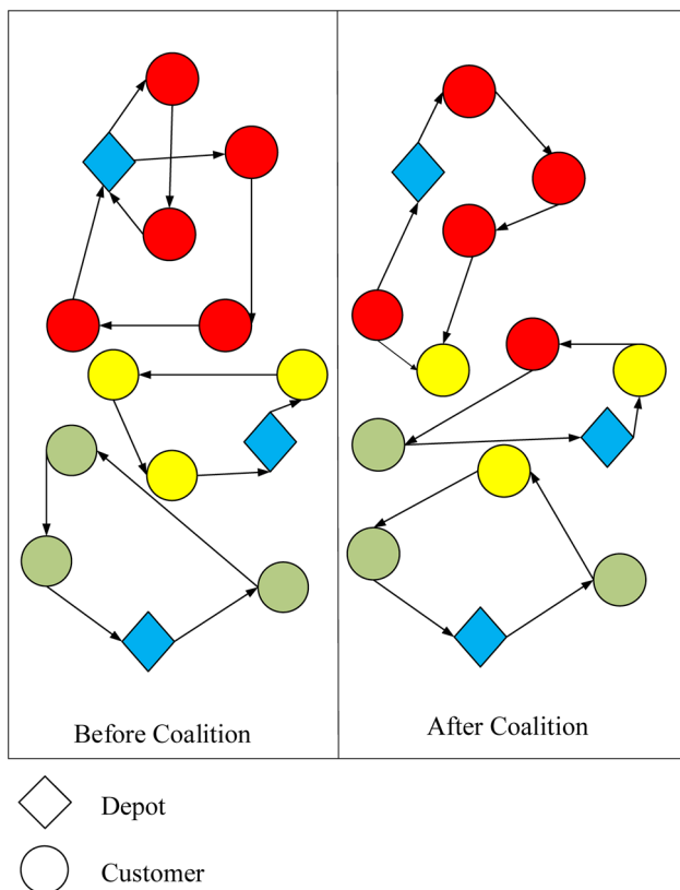
Fig. 1 Framework of CoMDVRP
