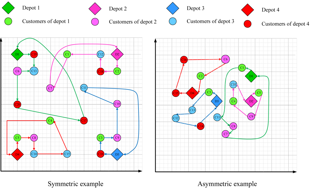
Fig. 3 Results of grand coalition in numerical examples
