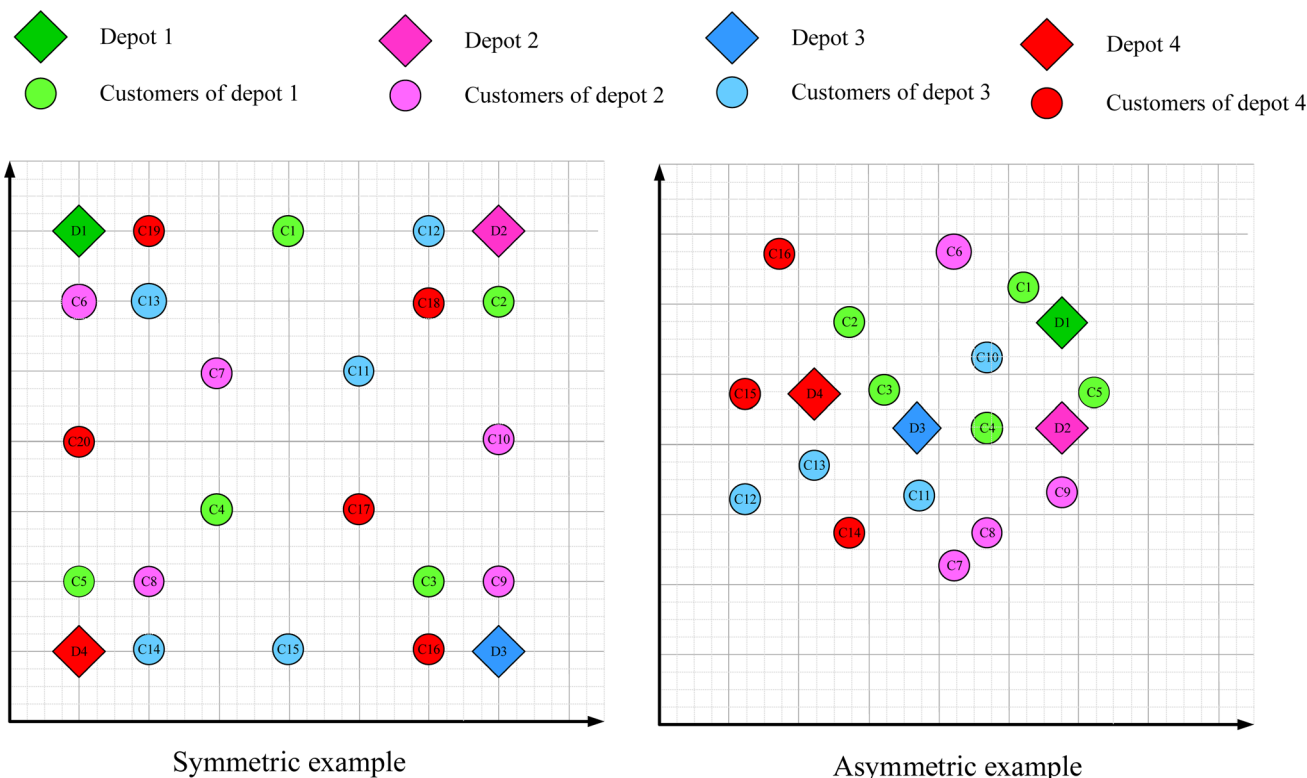
Fig. 2 Examples of coalition between 4 companies
