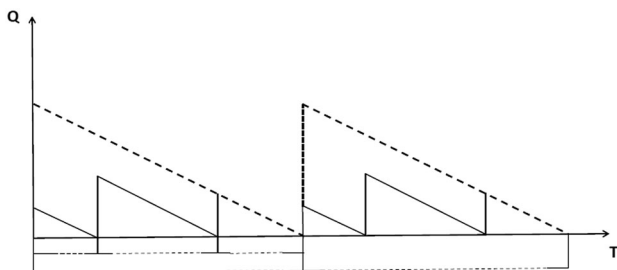
Fig. 1 Inventory behavior in the basic model
