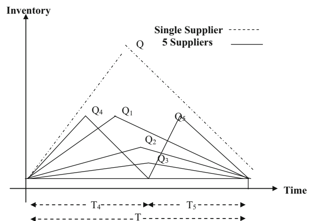
Fig. 2 Inventory behavior in Model A
