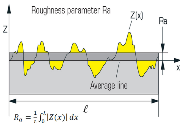
Fig. 1 The method used for calculation of SR (Azadi Moghaddam and Kolahan 2014)
