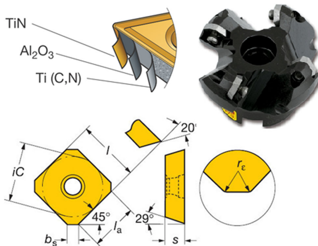
Fig. 3 Cutting tool used for machining
