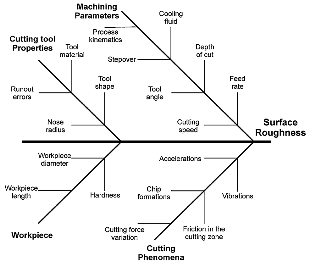
Fig. 2 Fishbone diagram with factors that influence on surface roughness (Baji et al. 2008)
