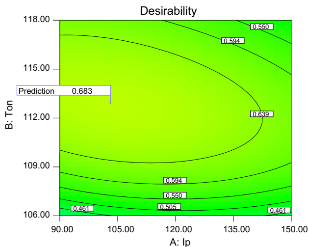
Fig. 7 Contour plot for overall desirability ( T_{off} : 37 μs; SV: 50 V)
