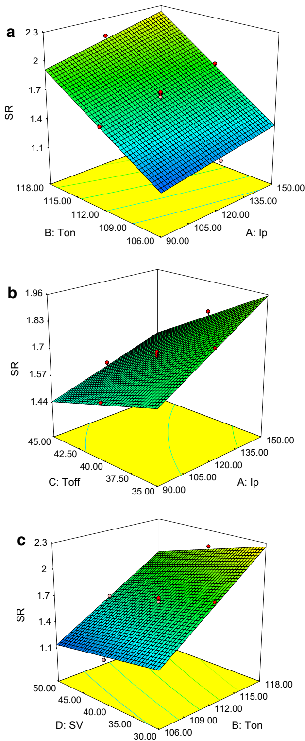
Fig. 4 a Effect of Ip and Ton on SR at Toff: 40 \mu s; SV: 40 V, b effect of Toff and Ip on SR at Ton: 112 \mu s; SV: 40 V, c effect of Ton and SV on SR at Ip: 120 A; Toff: 40 \mu s
