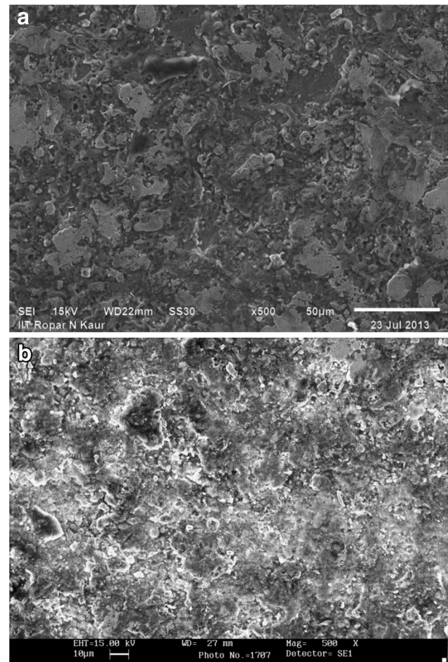
Fig. 5 a WEDM machined surface at Ip: 150 A; Ton: 118 \mu s; Toff: 35 \mu s; SV: 30 V, b WEDM machined surface at Ip: 90 A; Ton: 106 \mu s; Toff: 50 \mu s; SV: 50 V
