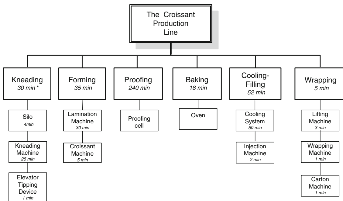
Fig. 3 A schematic presentation of croissant production line
