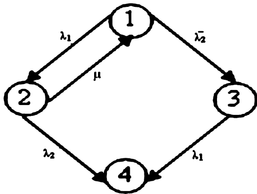
Fig. 1 Rate diagram for a standby system with repair
