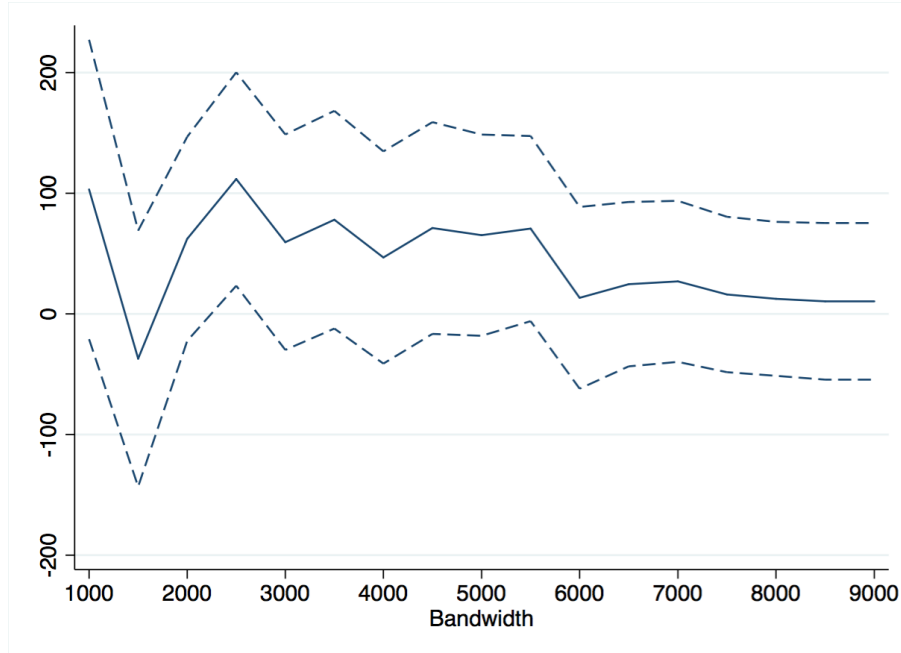
Figure 11: Local polynomial regression, p=1 . Sensitivity to the choice of bandwidth = 1000, ..., 9000.
