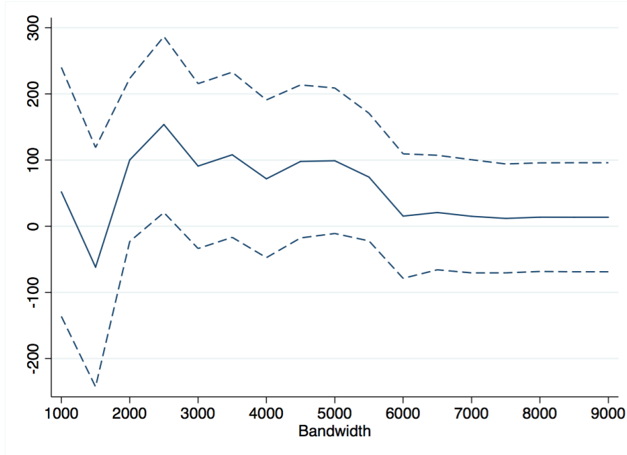
Figure 13: Local polynomial regression, p=1 . Cities only. Sensitivity to the choice of bandwidth = 1000, ..., 9000.
