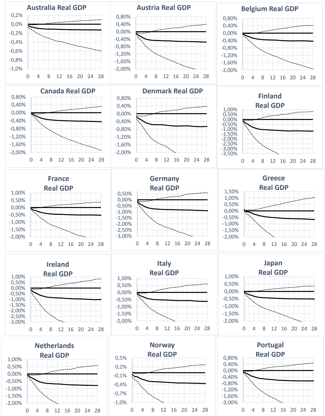
Figure 1. Generalized impulse responses of a negative unit (1 s.e.) shock to German government total expenditure (bootstrap mean estimates with 80% bootstrap error bounds)
