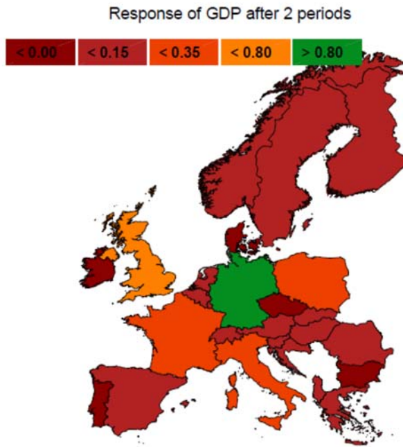
Figure 7. Spillover reactions after a German government spending shock (Georgiadis/Hollmayer)
