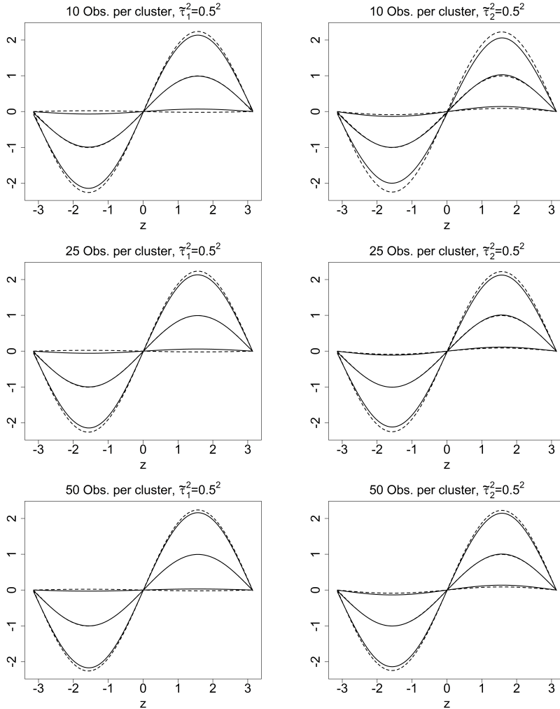
Figure 8: The average estimates of the functions f_l(z) as well as of the smallest and largest district-specific effects (1 + \alpha_{cl}) f_l(z) (solid) and the respective true effects (dashed) for the Gamma Models 1 to 3. The first column shows the effects of the \mu -parameter, the second column those of the \sigma -parameter.
