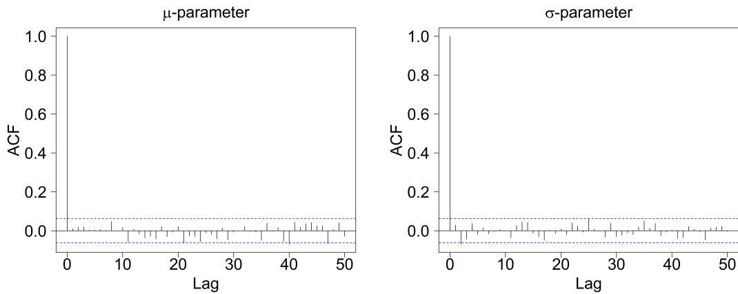
Figure 4: Autocorrelation functions of the random effects \alpha_{cl} of the district of Munich in one of the replications of the Gaussian Model 1.
