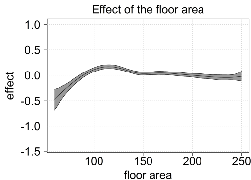
Figure 24: Average marginal effect of the floor area for the shape parameter in the Gamma model together with simultaneous 95% confidence bands.
