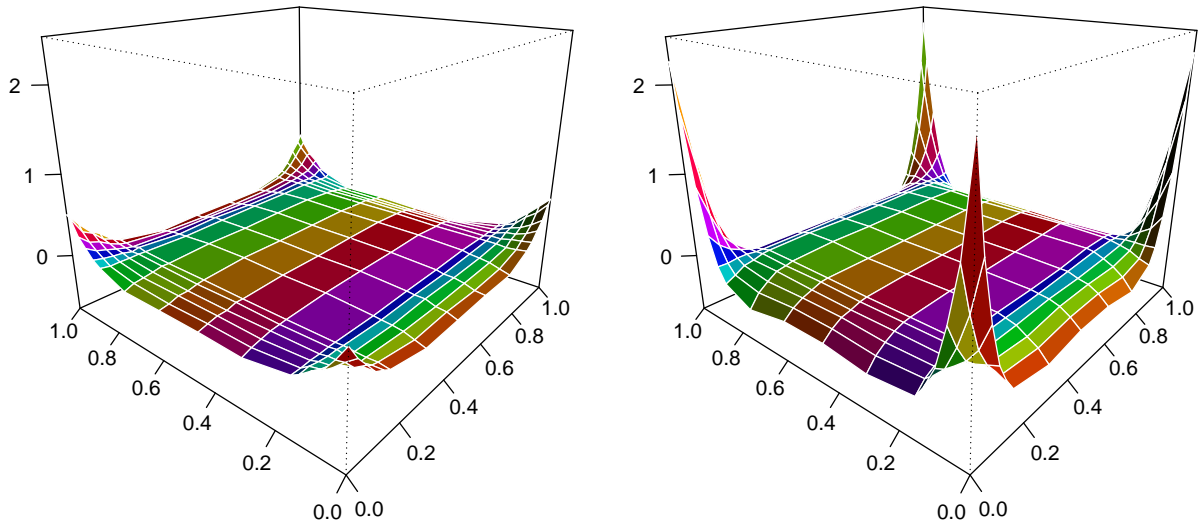
Figure 3: Simulated influence function (1,000 iterations) of T_\alpha for \alpha = 1 (left) and \alpha = 3 (right) for a bivariate sample of size n = 50 with independent, uniformly distributed margins.
