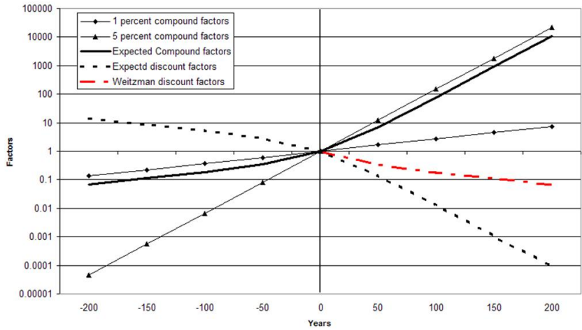
Figure 2 Compound factors at 1% and 5%, their expected value and the corresponding discount factors, logarithmic
