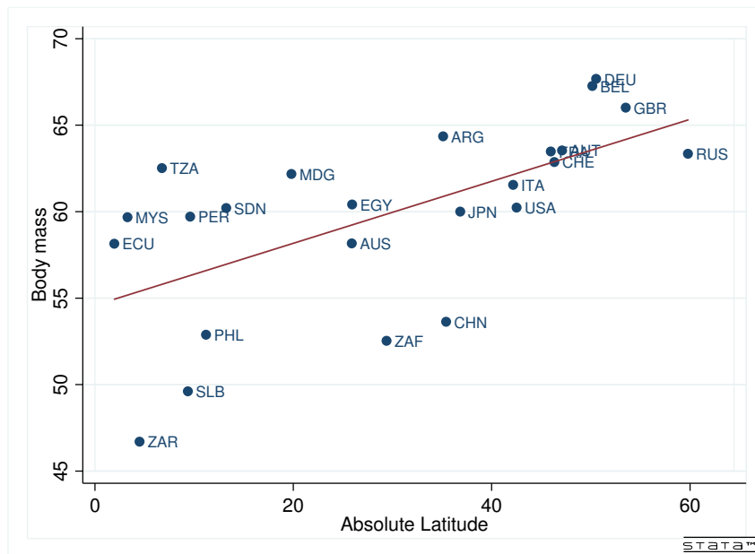
Figure 3: Bergmann’s Rule
