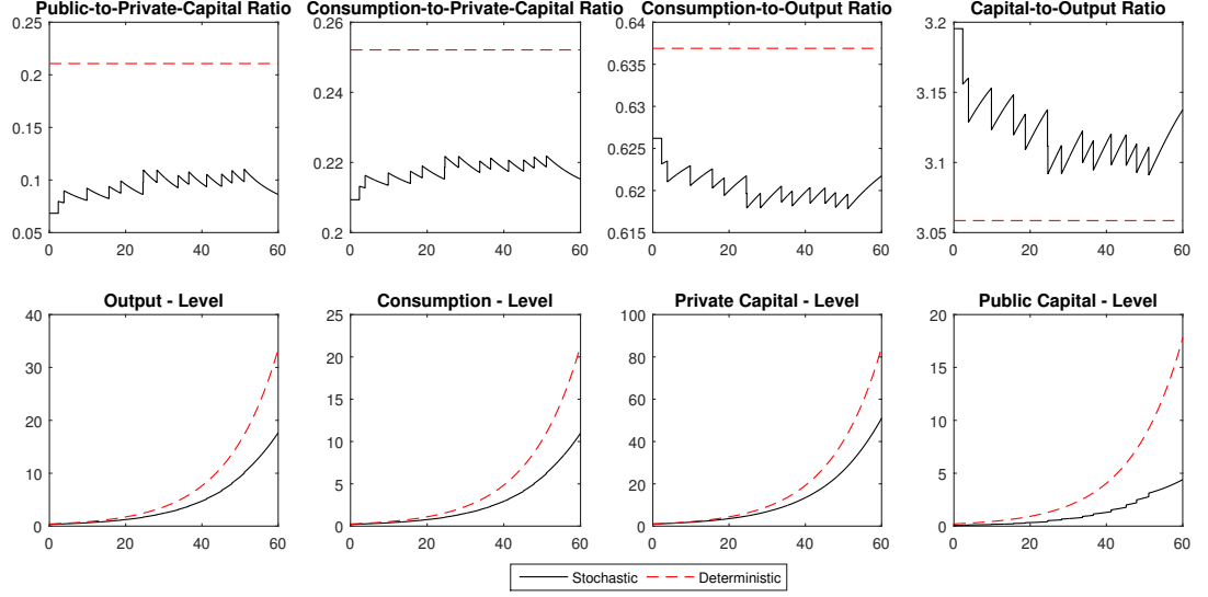
Figure 5: Transition Paths: Deterministic and Stochastic Models.
