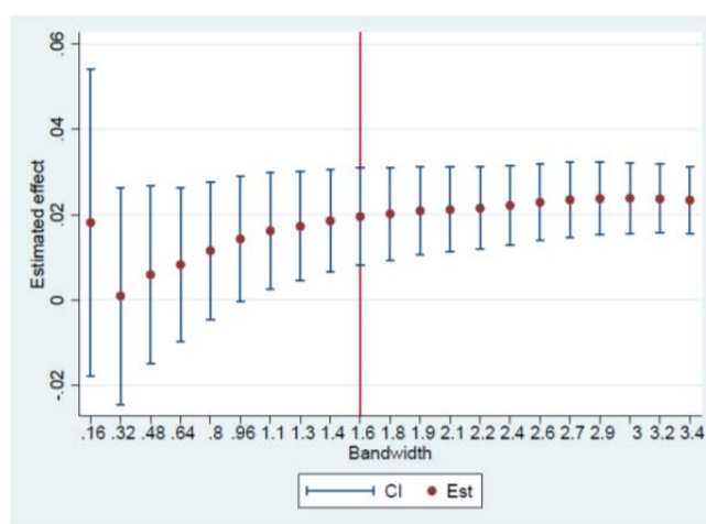
Figure 9: The RD estimate of the threat effect as a function of bandwidth
