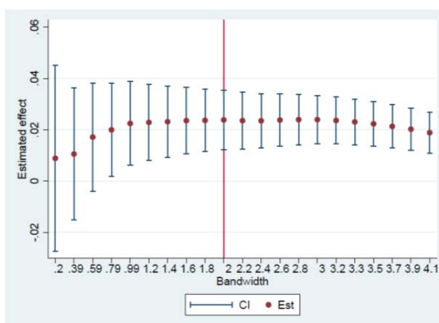
Figure 10: The RD estimate of the effect during day 1-180 as a function of bandwidth
