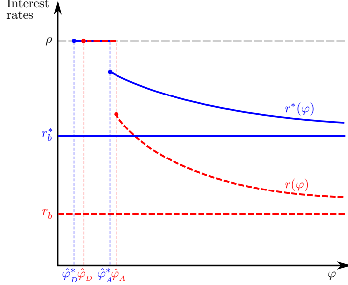
Figure 3: The structure of interest rates when liquidity is scarce in all OTC matches
