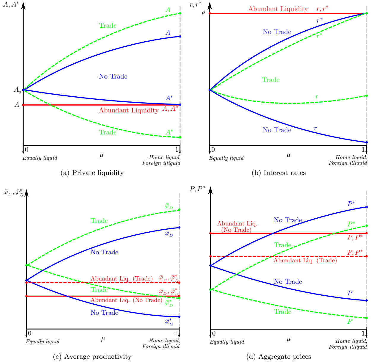
Figure 4: The impact of differences in financial development and the unequal effects of trade
