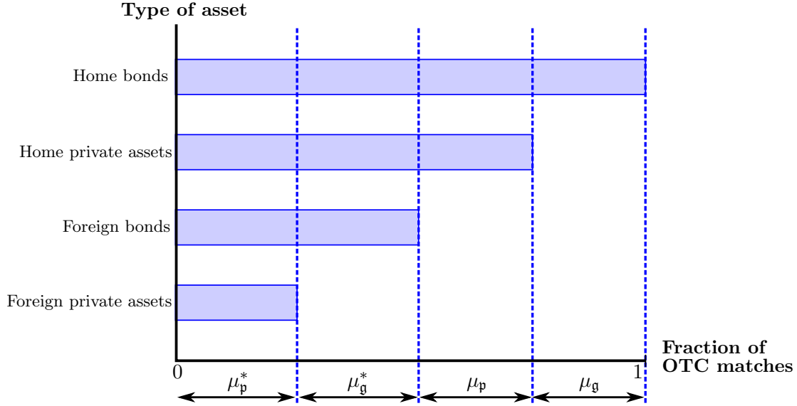
Figure 2: Acceptability of Home and Foreign assets in OTC matches
