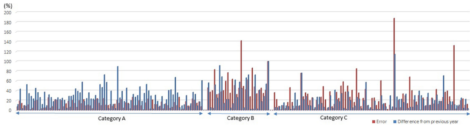
Figure 12 Forecast error rates and the differences from the previous year for 200 alternators.
