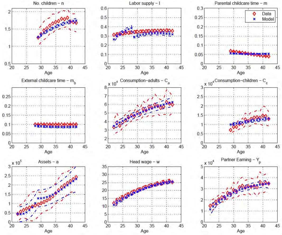
Figure 2: Fitting the model to the US data
