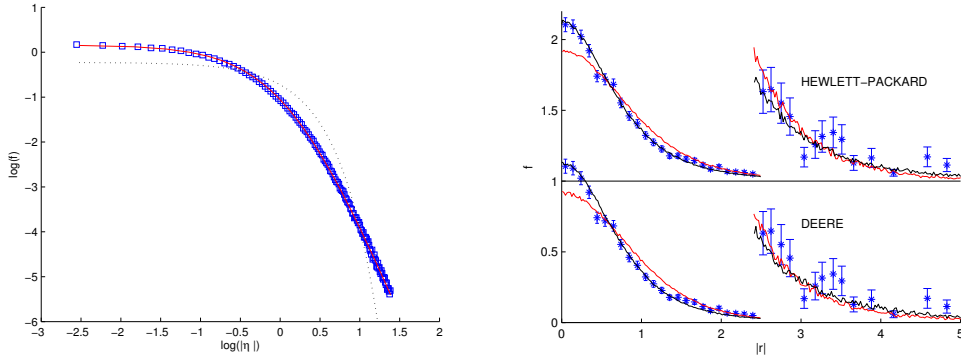
Figure 1: The left panel shows the pdf of all GARCH filtered returns \eta_G(t)_i obtained from the raw returns by equation (22). The red line corresponds to a fitted t-distribution with \nu = 3.32 , the dotted line shows a Gaussian distribution. In the right panel two typical pdfs for stocks of the S&P market are compared with the predicted pdf using t-distributed (black) or Gaussian (red) noise. The values (log of the pdf) |r| > 2.5 are multiplied by a factor of 10.
