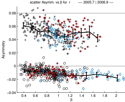
Figure 10: Asymmetry of r vs \bar{\beta} for stocks. Blue diamonds refer to technology, red stars to financials. The line corresponds to average \bar{\beta} and stdev.
