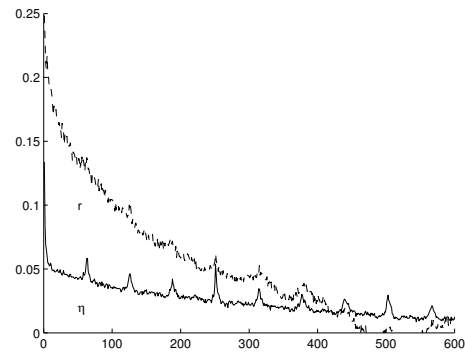
Figure 3: Autocorrelation for returns |r_{ti}| averaged over all stocks (top) and the averaged GARCH filtered returns |\eta_G(ti)|
