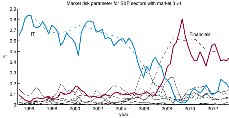
Figure 9: Time dependence of the risk parameter described in equation (24) for the sectors of the S&P market. The dashed line shows the result of Raddant and Wagner (2017). The solid lines (blue for the information technology and red for the financial sector) use daily \beta s from the RMG.
