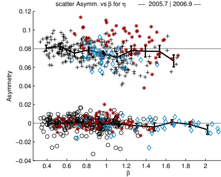
Figure 11: Asymmetry of \eta vs \bar{\beta} for stocks. Blue diamonds refer to technology, red stars to financials. The line corresponds to average \bar{\beta} and stdev.
