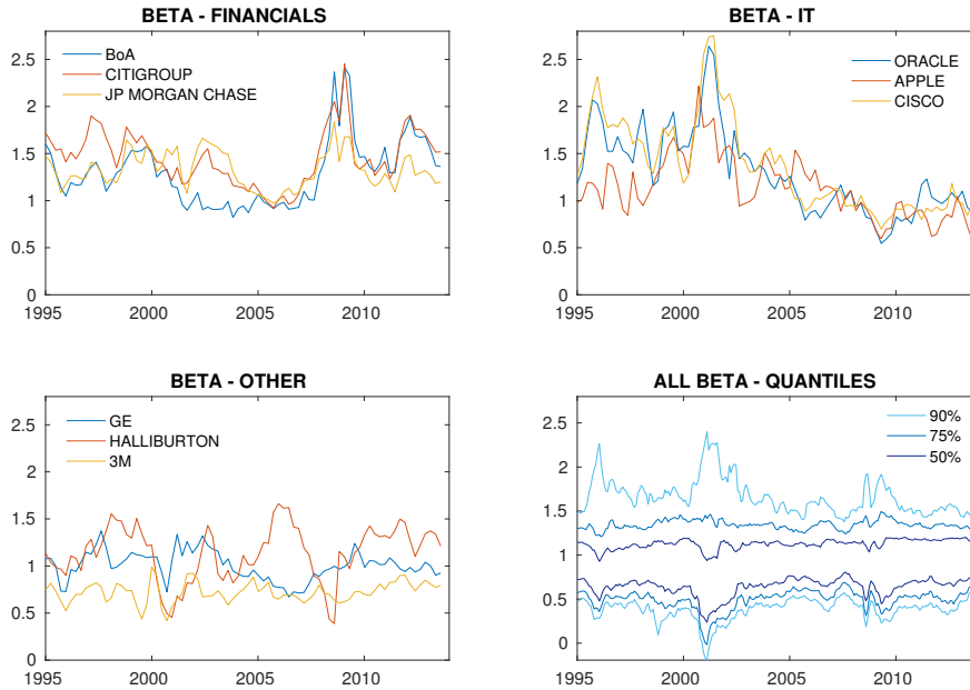
Figure 4: Beta values from the RMG model. The top and the bottom left panel show beta values for different stocks, averaged over a 60-day window. The bottom right panel shows the dynamics of the distribution of beta values by the quantiles, using a 20-day window.
