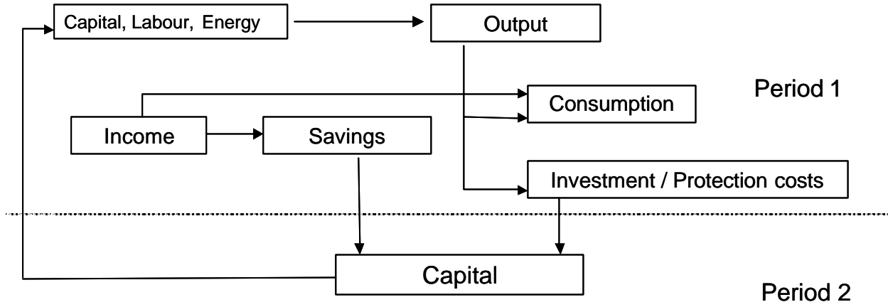
Figure 3: Dynamic structure
