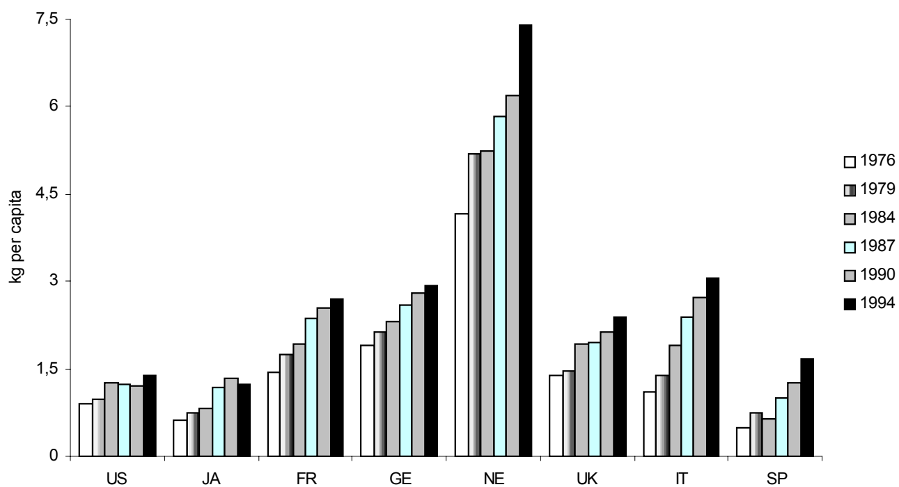
Figure 9. SO 2 . Embodied Emissions in Imports Over Time
