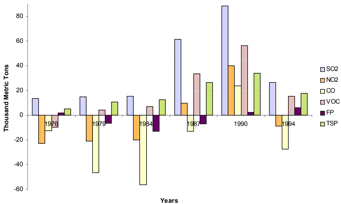
Figure 2. Western Europe. Balance of Embodied Emissions in Trade
