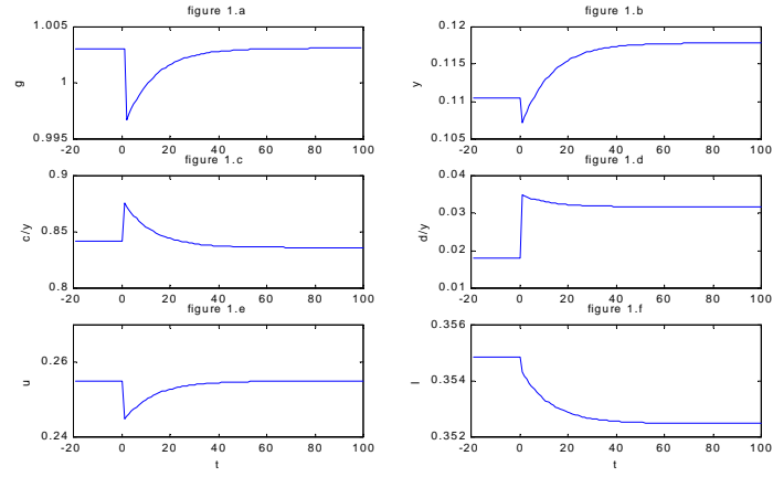
Figure 1: Transitional dynamics 1
