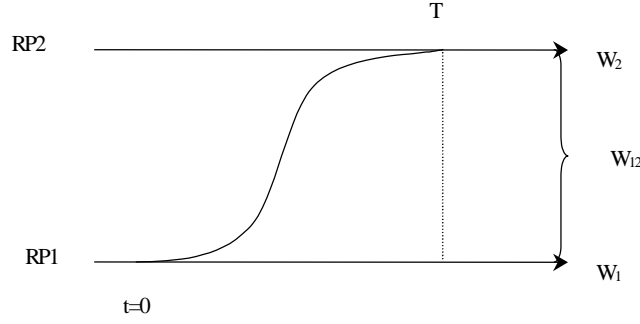
Figure 3: Welfare decomposition
