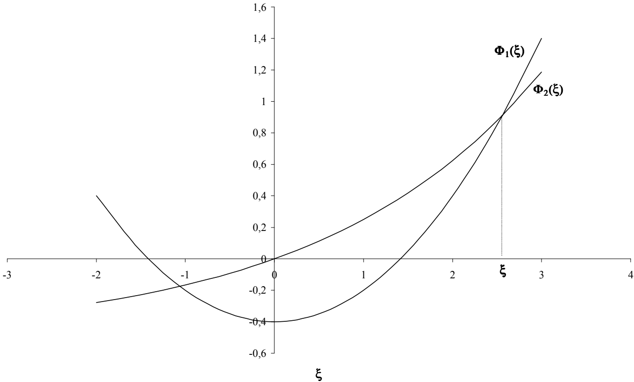
Figure A1 - Solution for \xi . with \phi > 0
