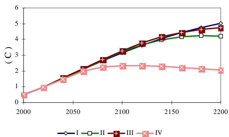
FIGURE 5. Global mean temperature increase, relative to the pre-industrial level, for the period 2000-2200.
