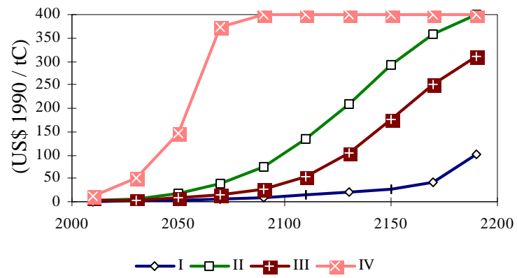
FIGURE 2. CO 2 emission price, for the period 2000-2200.
