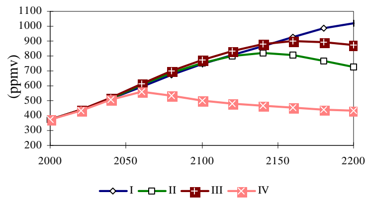
FIGURE 4. CO_2 concentration, for the period 2000-2200.
