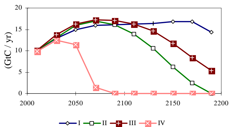
FIGURE 3. Net CO 2 emission, for the period 2000-2200.
