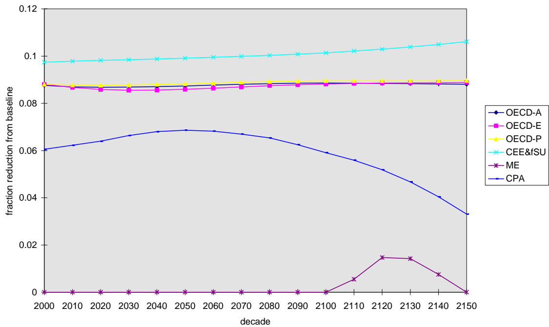
Figure 6. The regional and temporal distribution of emission reduction efforts for the no-envy control case.
