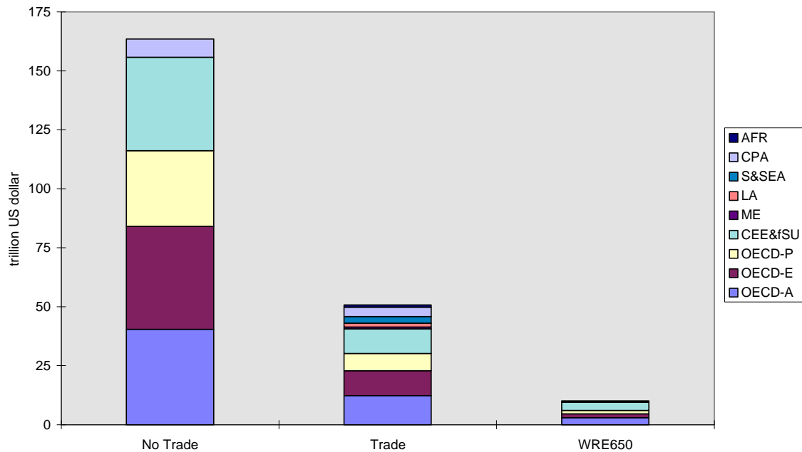
Figure 7. Consumption losses in the period 1990-2200, discounted to 1990 at 5% per year, due to emission reduction for two no-envy emission control scenarios without and with international trade in emission permits and the WRE scenario without international trade and concentration in the long run.
