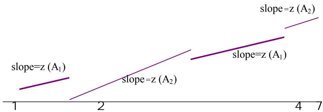
FIGURE 3: UCE with non-interval jurisdictions
