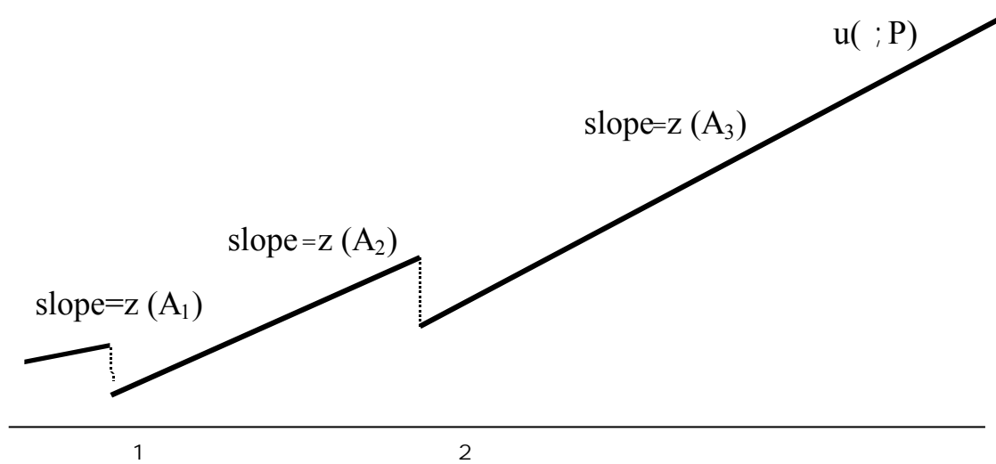
FIGURE 2: Utilities in UCE and ET
