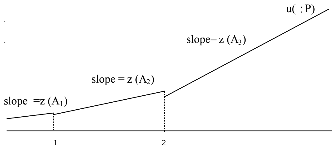
FIGURE 1 Utilities in Free Mobility Equilibrium
