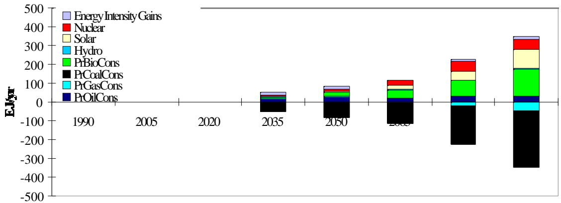
Figure 7. The OGF Global Energy System: Reference, Protocol, and Changes
