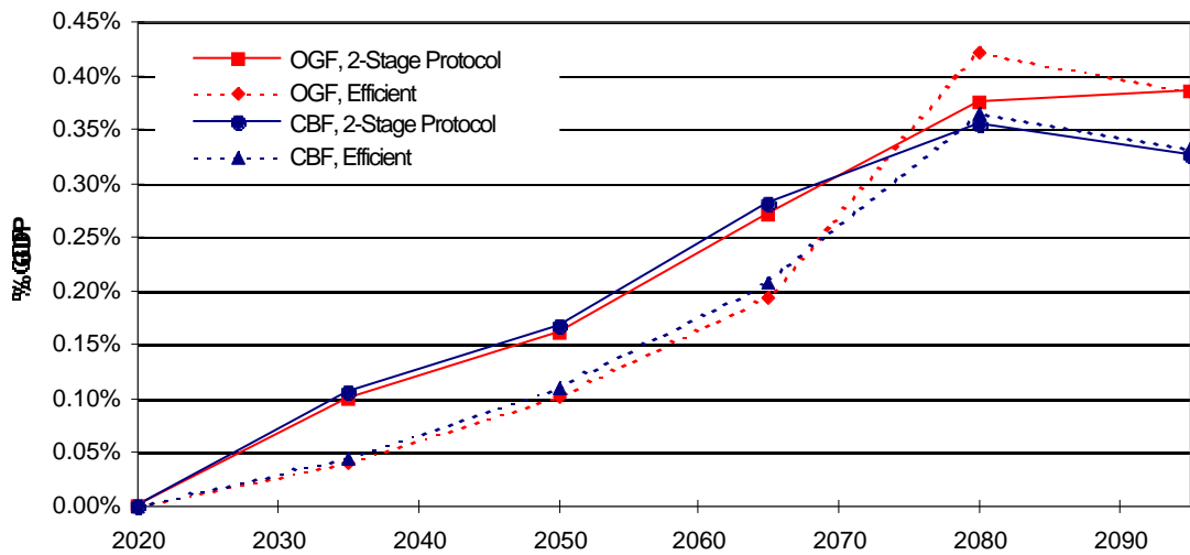
Figure 11. Comparison of Technology Protocol to Efficient Mitigation: Global Annual Costs
