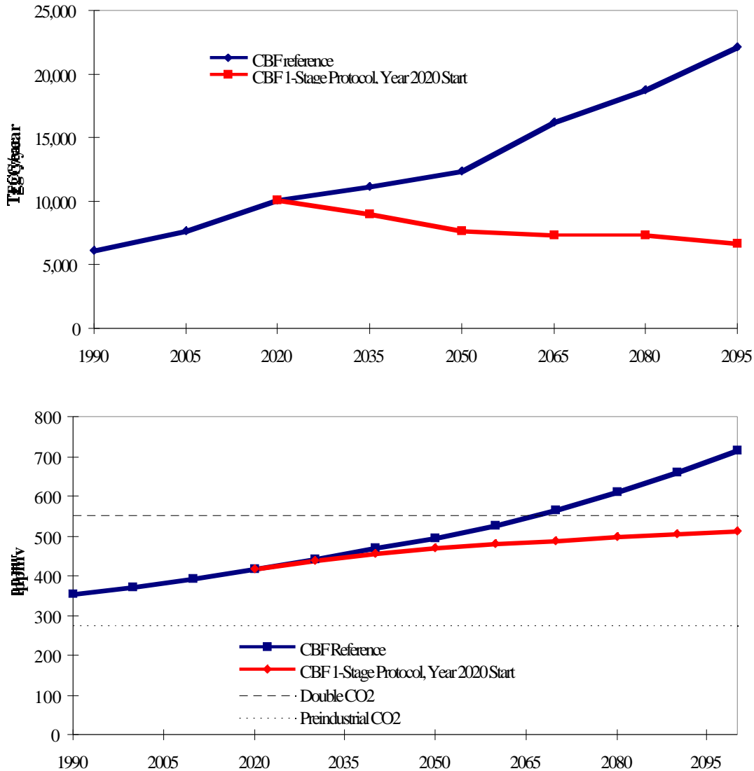
Figure 6. CBF: Global Carbon Emissions and CO 2 Concentrations
