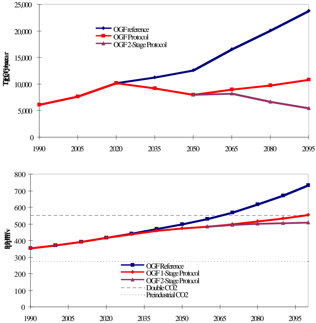
Figure 8. OGF: Global Carbon Emissions and CO 2 Concentrations
