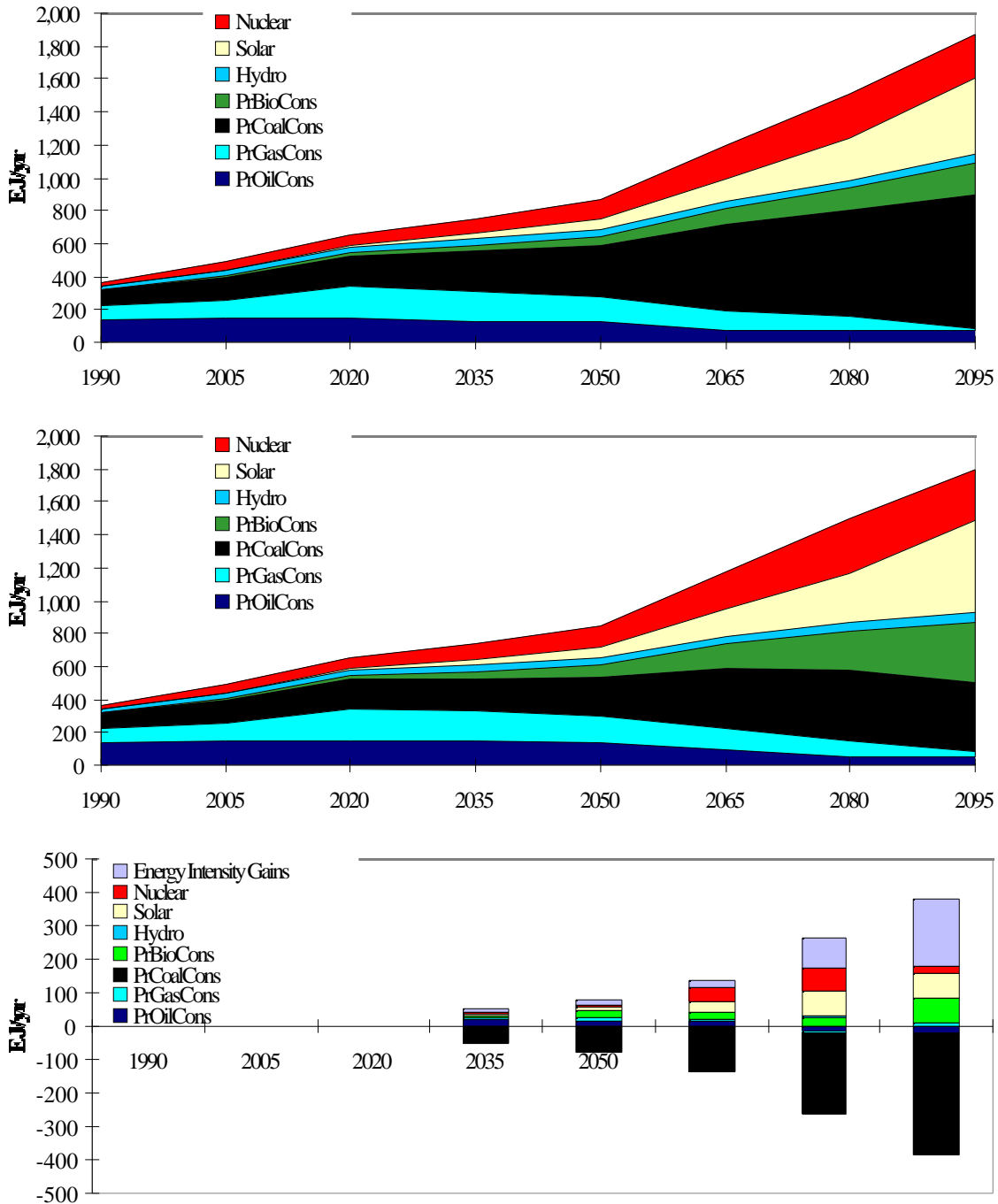
Figure 5. The CBF Global Energy System: Reference Case, Protocol, and Changes
