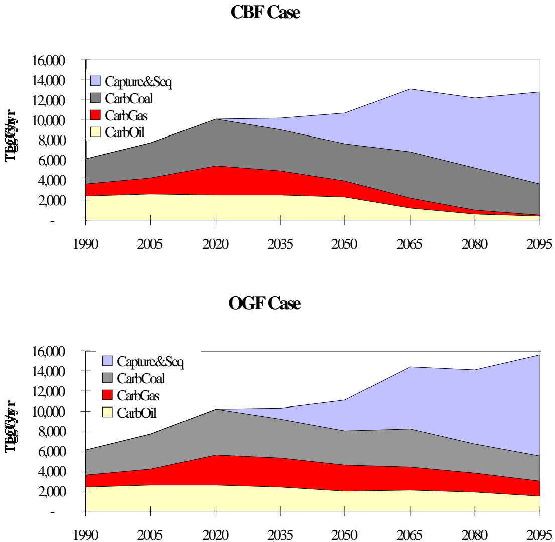
Figure 9. Global Carbon Emissions by Fuel, Capture and Sequestration
