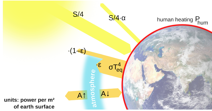
Figure 10: Single layer atmosphere with human heating P_{hum} . The albedo \alpha indicates the fraction of incoming sunlight reflected immediately. At the Earth's crust, a layer of human heat emissions is added. Earth's infrared emissions are due to black body radiation, and a fraction \epsilon is absorbed in the atmosphere and radiated evenly in both directions.
