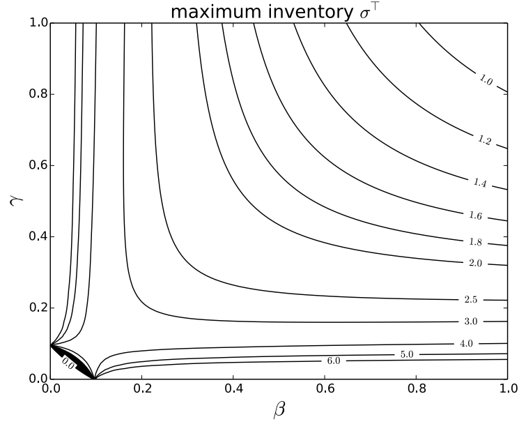
Figure 6: Contour plot of instability induced by inventory oscillations, depicting the maximum possible inventory to expected sales ratio \sigma^\top in order to keep the fixed point stable. In the lower left corner, no stable fixed point exists for any \sigma^\top \geq 0 .
