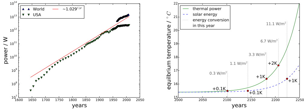
Figure 11: Left: energy conversion in the USA and the world, data from BP (2009) and Energy Information Administration (2012a,b). The solid line indicates an exponentially growing curve with a yearly growth rate of 2.9%. Right: equilibrium temperature of planet Earth calculated by (68), assuming continued exponential growth of energy conversion. The dashed line corresponds to the use of solar energy with the effective albedo \alpha_{eff} .
