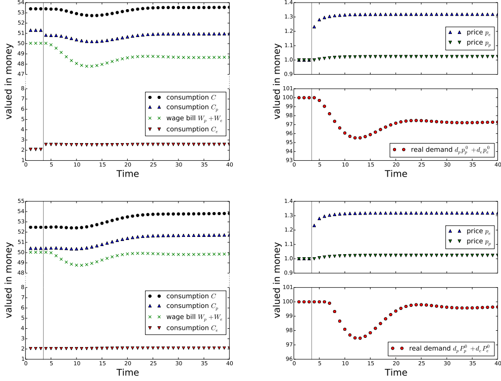
Figure 7: Impact of an increase in energy markup \phi_e : We initiate the model at the fixed point calculated in section 4.2, and the vertical line indicates the time when the markup on energy is exogenously increased. The left plots shows the decrease of consumption that causes a reduction of demand, which drives down wages and further reduces consumption. The upper two plots keep government expenditures fixed in nominal terms, while the lower plots adapt to price inflation. The right plots indicate the increase in prices caused by the higher energy markup, and the time evolution of real demand, showing a significant temporary decline which is permanent only in the case of nominally fixed government expenditures.
